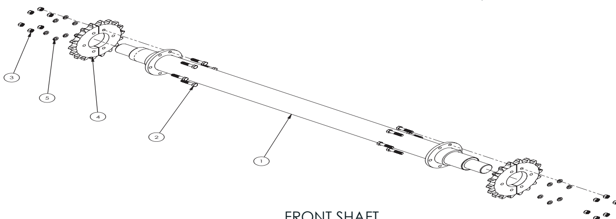
FRONT SHAFT
