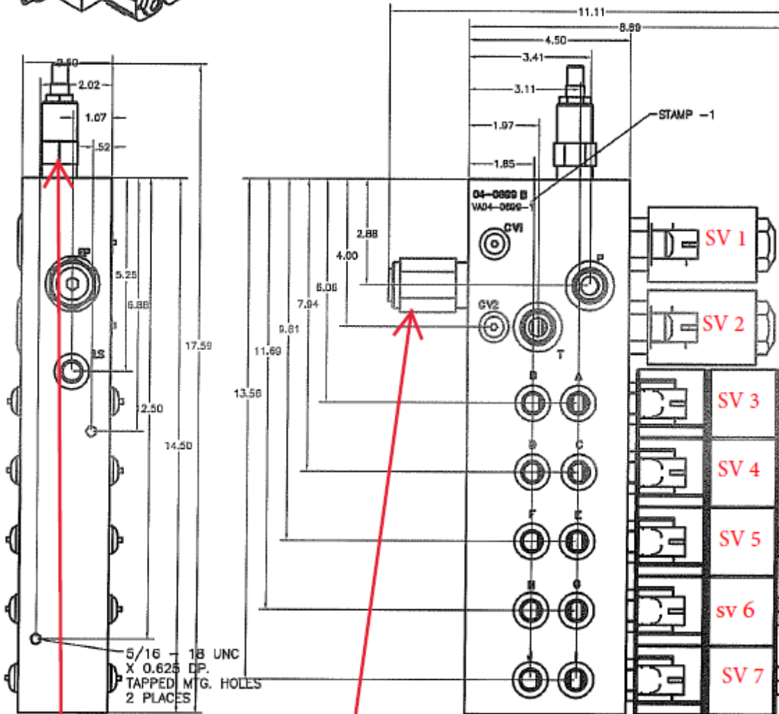
EP VALVE LOCATION (EARLY STYLE SHOWN P/N: 71.P291114)
