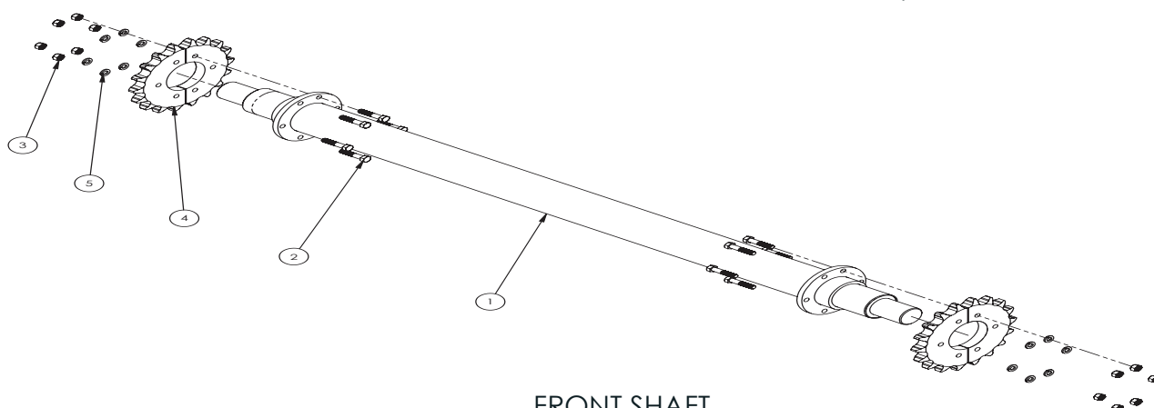
FRONT SHAFT
