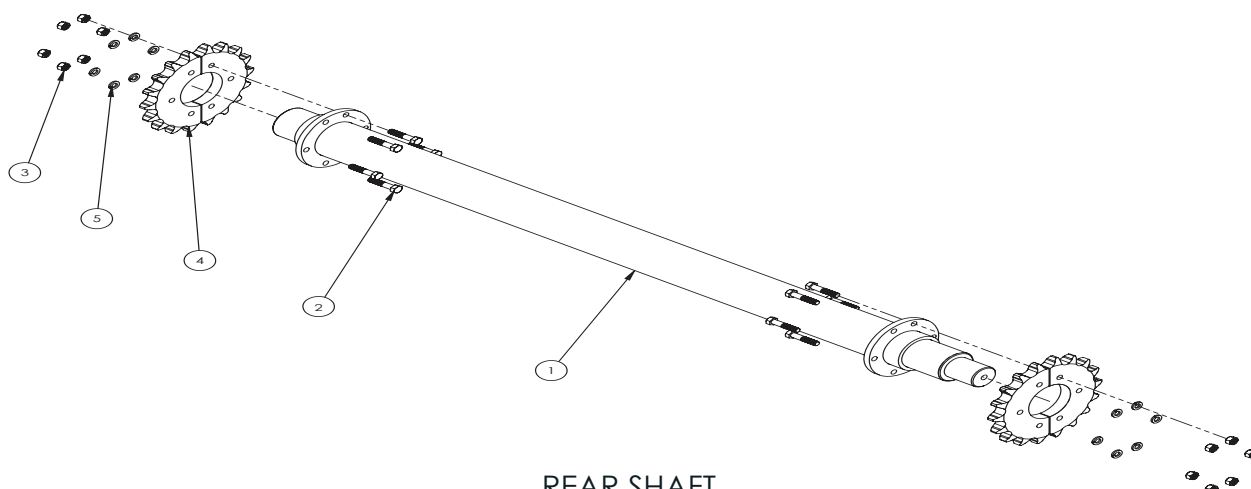
REAR SHAFT
