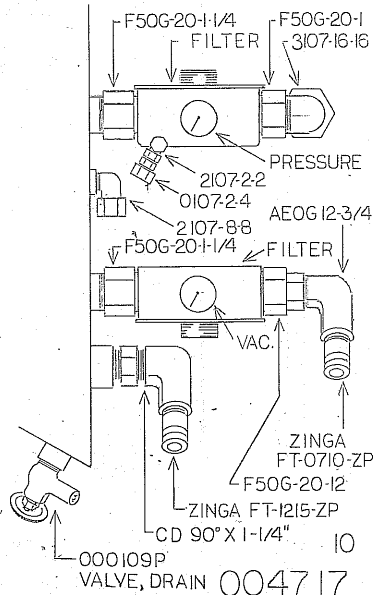
SIDE VIEW
